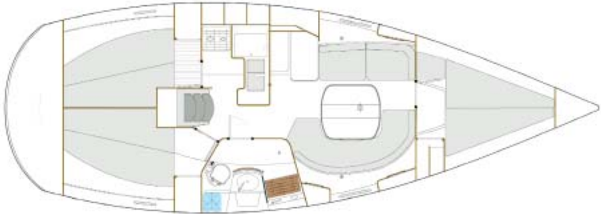
3 CABIN VERSION
