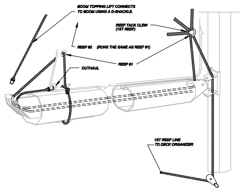
BOOM WITH REEFING LAYOUT
