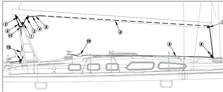
DUAL ENDED MAINSHEET PURCHASE LAYOUT
