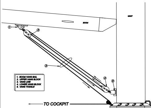
ROPE VANG DETAILS (STANDARD)
