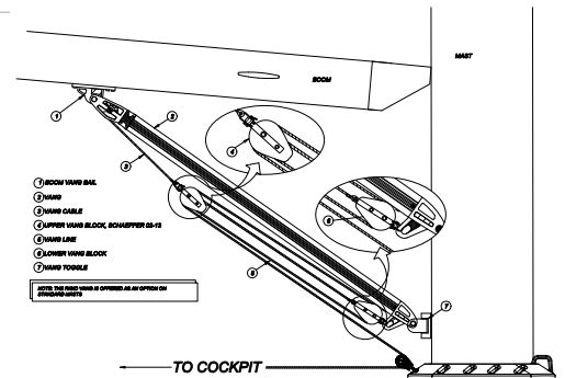
RIGID VANG (FURLING OPTION)
