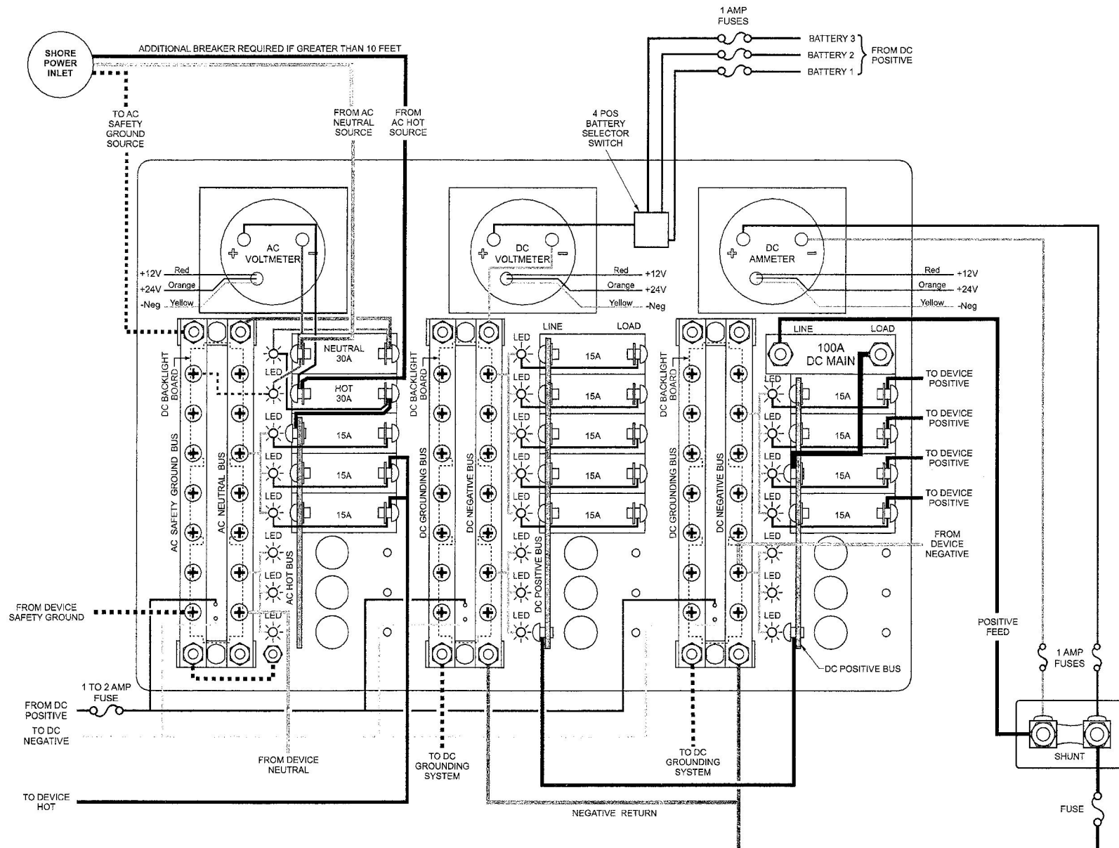
Wiring Diagram AC/DC Power Distribution Panel PN 8084 / PN 3084 shown for reference
